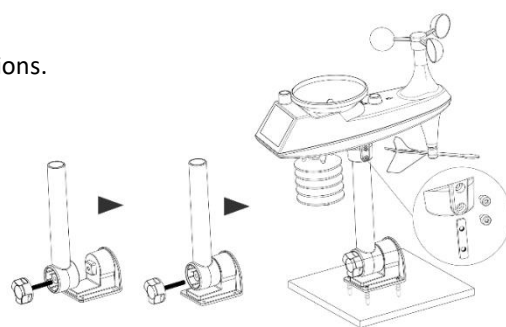
Installation method 1
