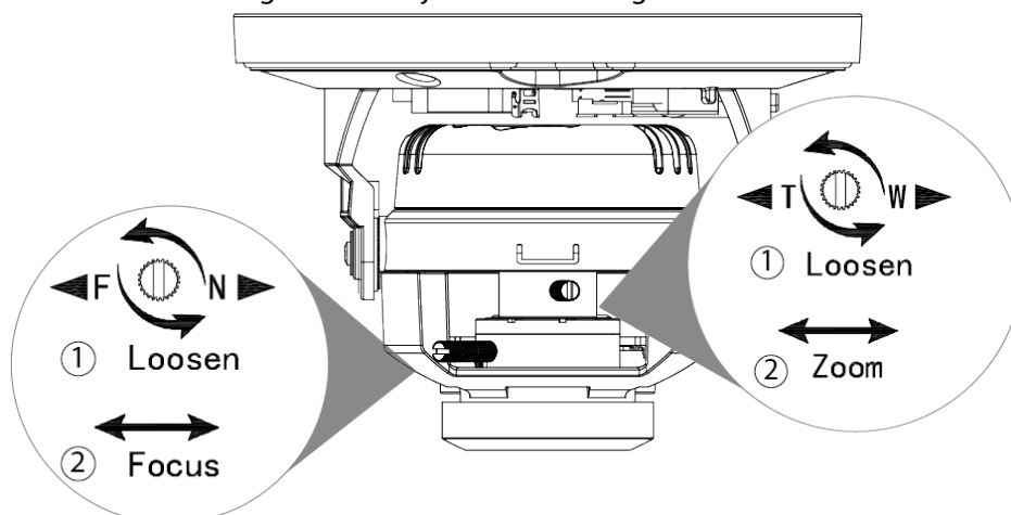
Figure 3-12 Adjust the focal length
