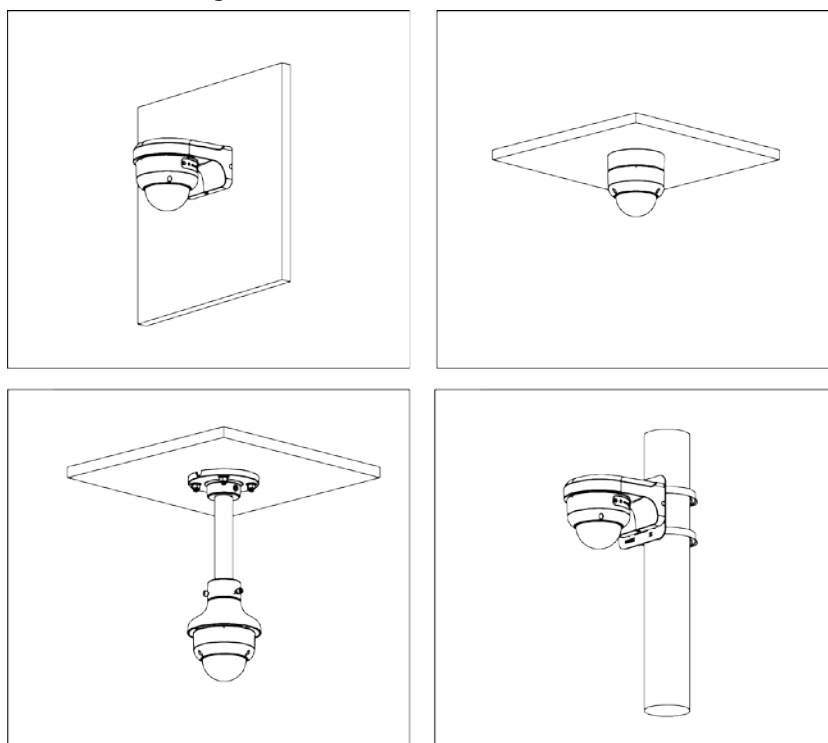
Figure 3-3 Installation method
