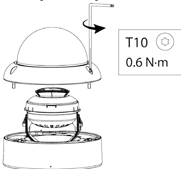
Figure 3-5 Detaching camera
