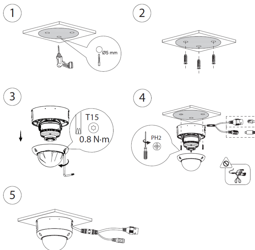
Figure 3-4 Cable going through the side cable tray
