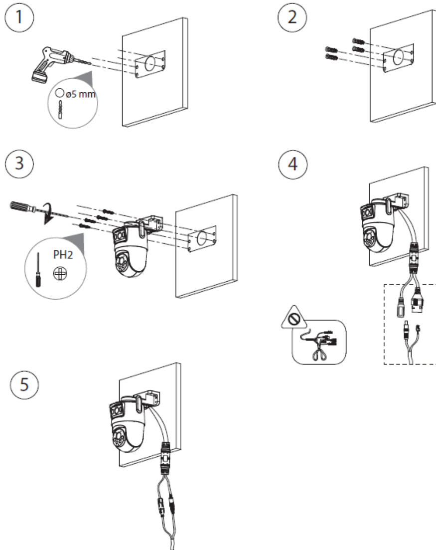
Figure 4-3 Wall mount
