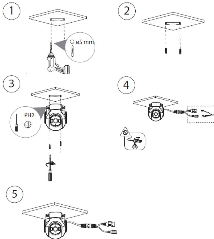
Figure 4-4 Ceiling mount
