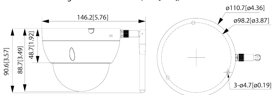
Figure 4-2 Dimensions (mm [inch])
