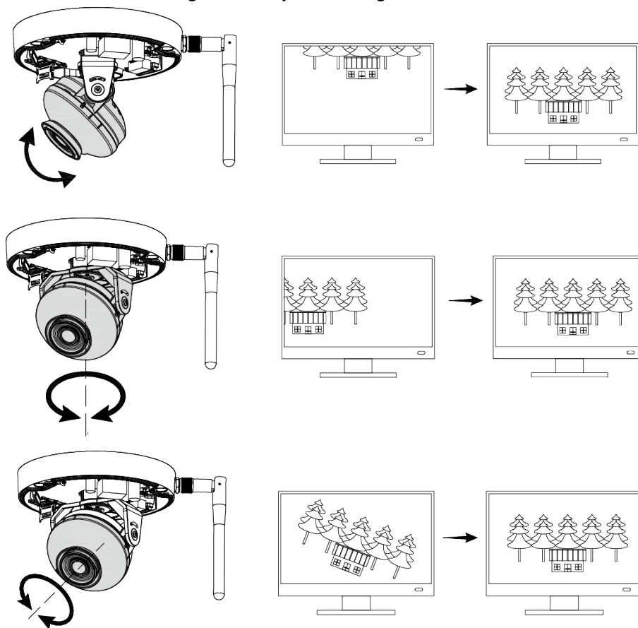
Figure 4-8 Adjust lens angle
