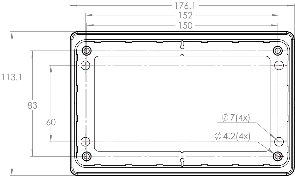
Frame dimensions
