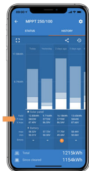
VictronConnect history Pmax
